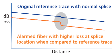
How an OTDR detects a tapped splice location
